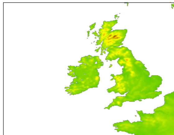
(c) COSMO-CLM 6 km
