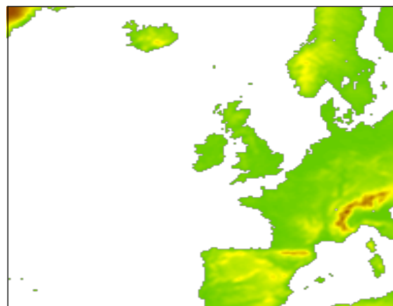
(a) COSMO-CLM 18 km
