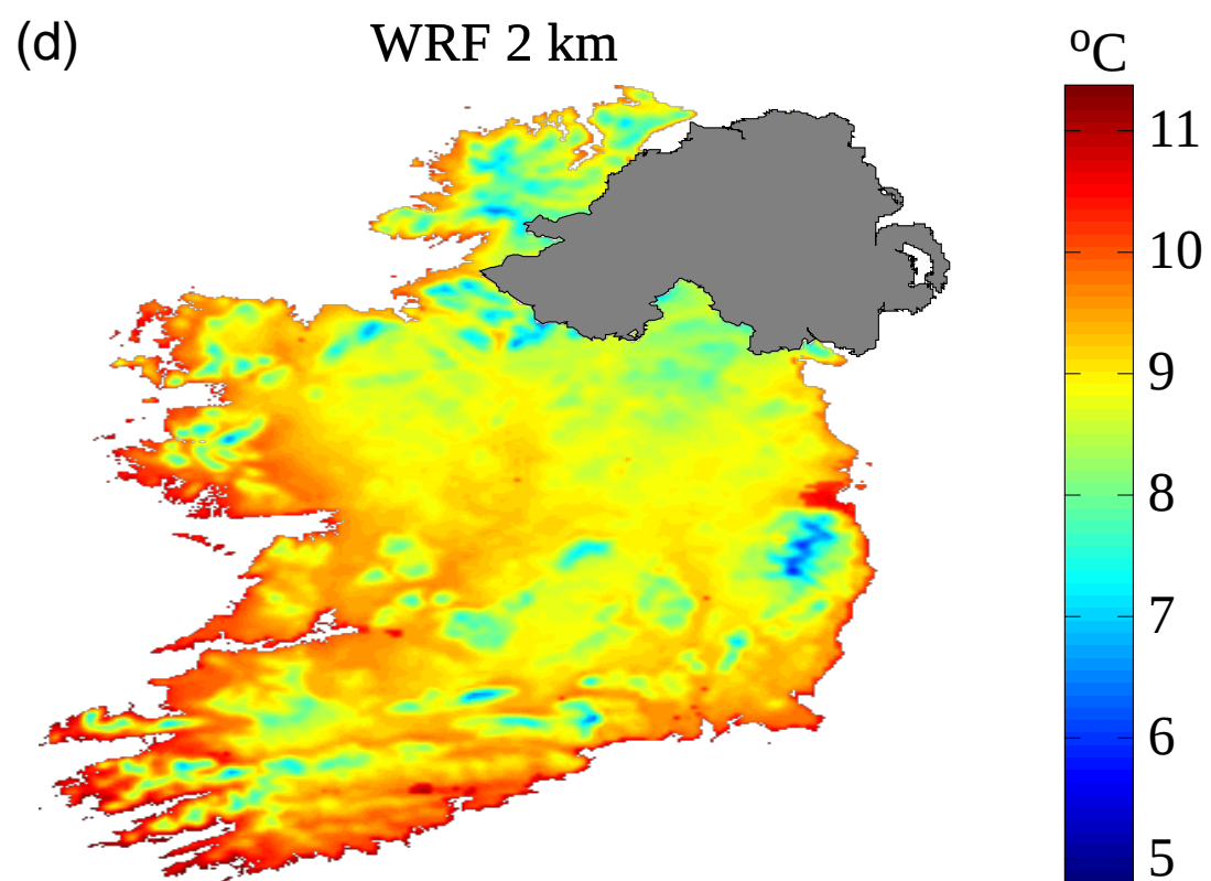
Average annual 2 m temperature (°C), 1981–2015
