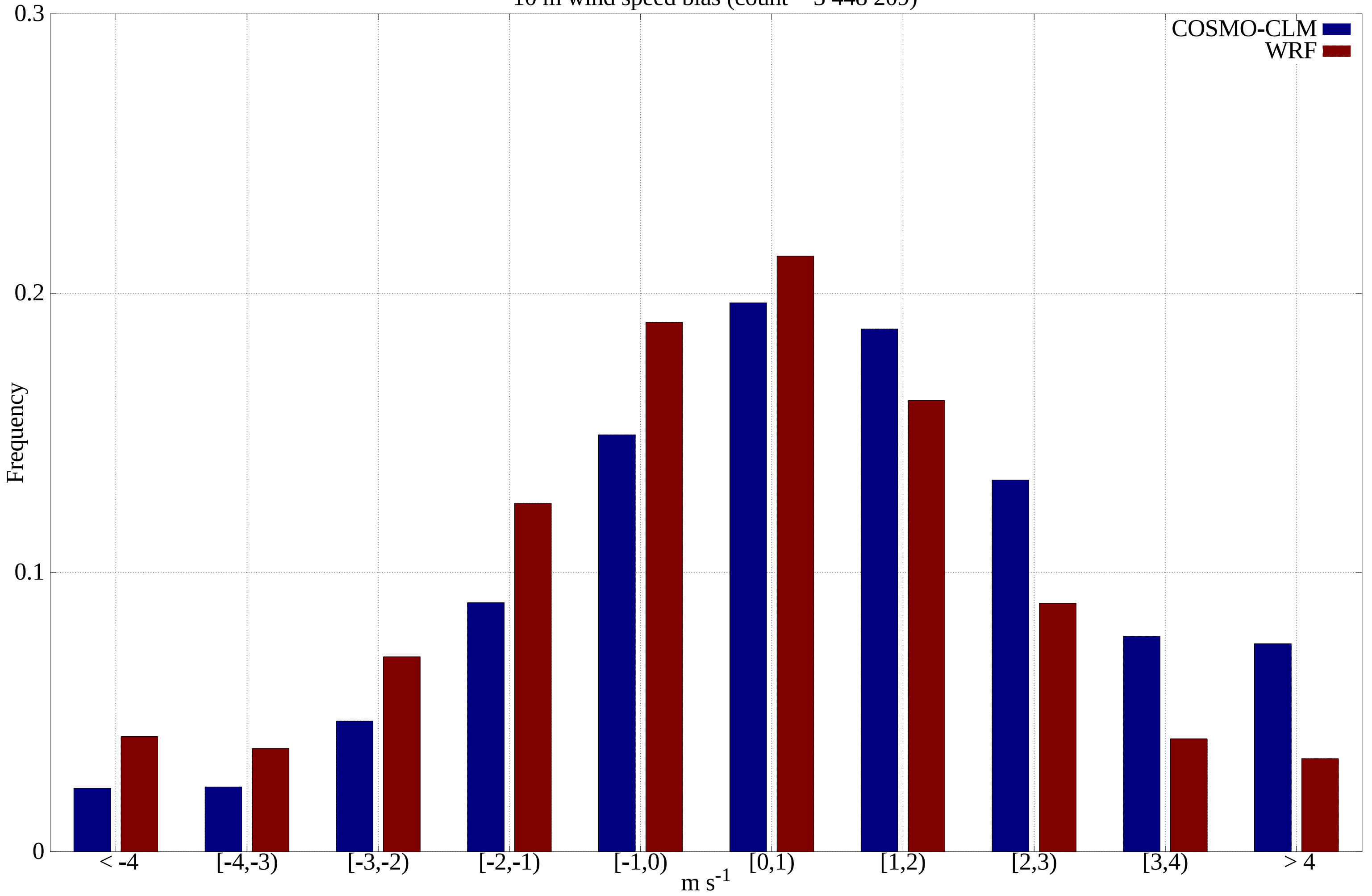
10 m wind speed bias (count = 3 448 209)
