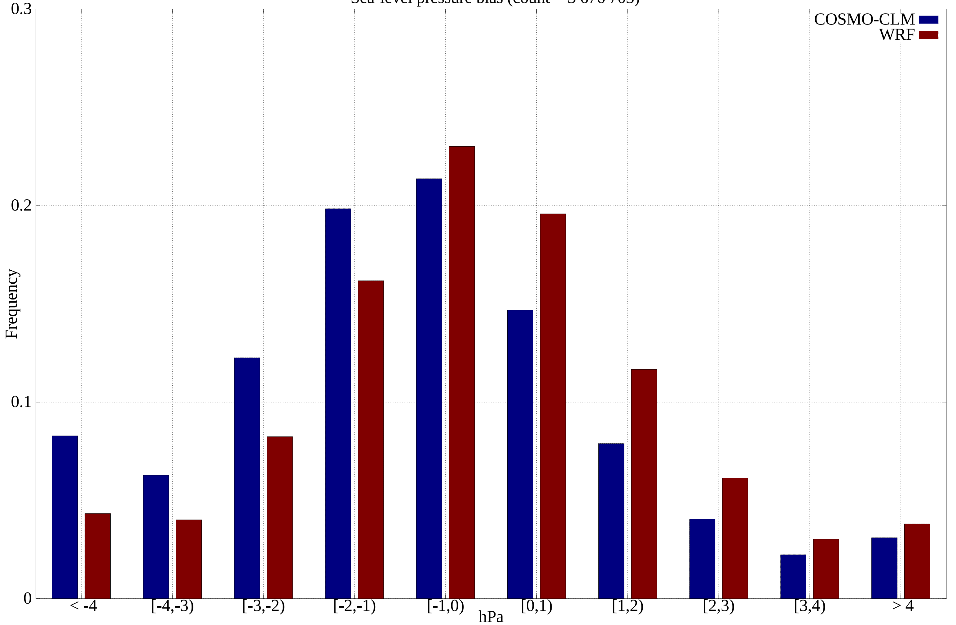
Sea-level pressure bias (count = 3 676 703)
