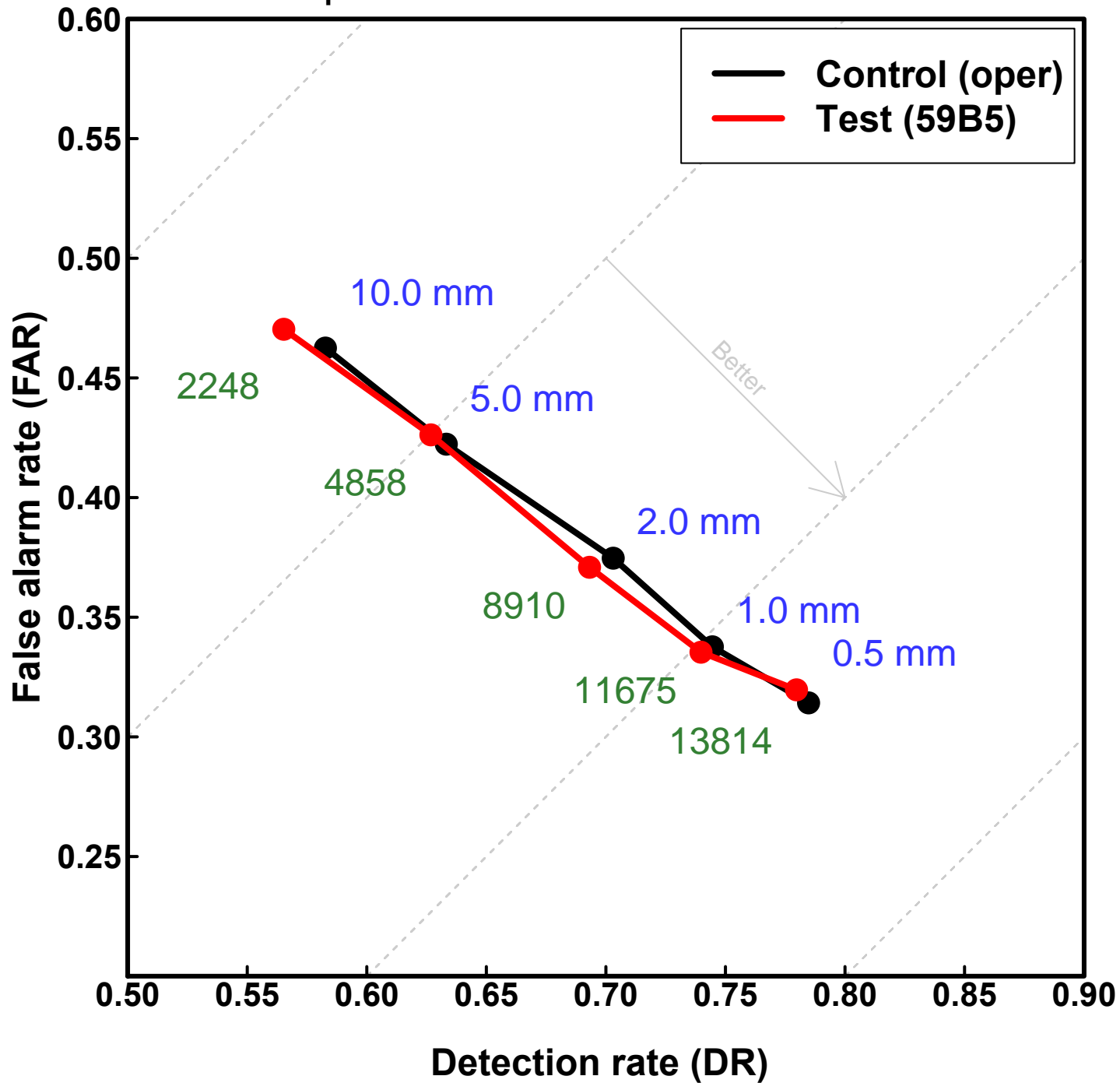
Precipitation scores for 12 h rain in AROME-France
