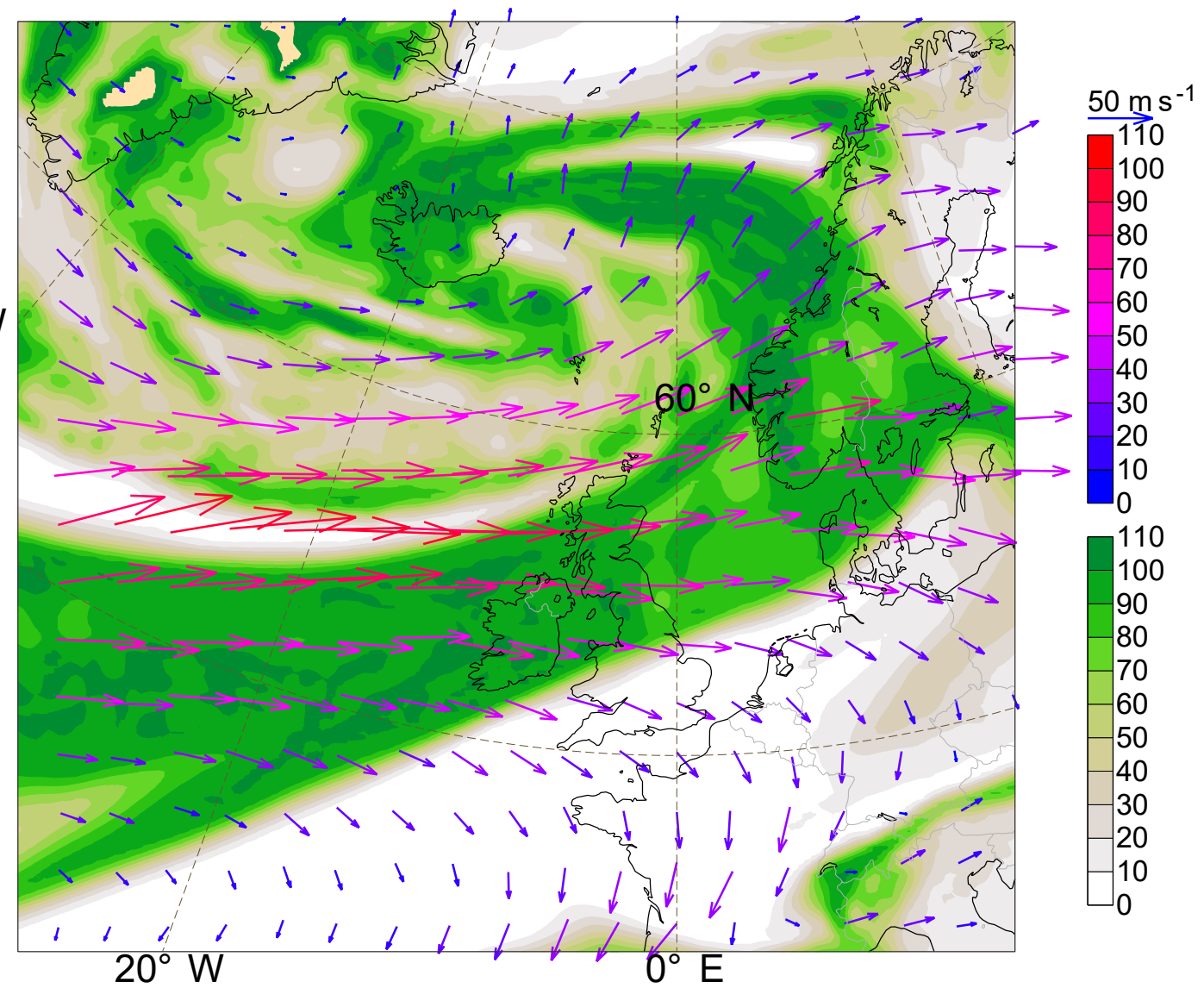
(b) T639L137 OpenIFS; t+27
