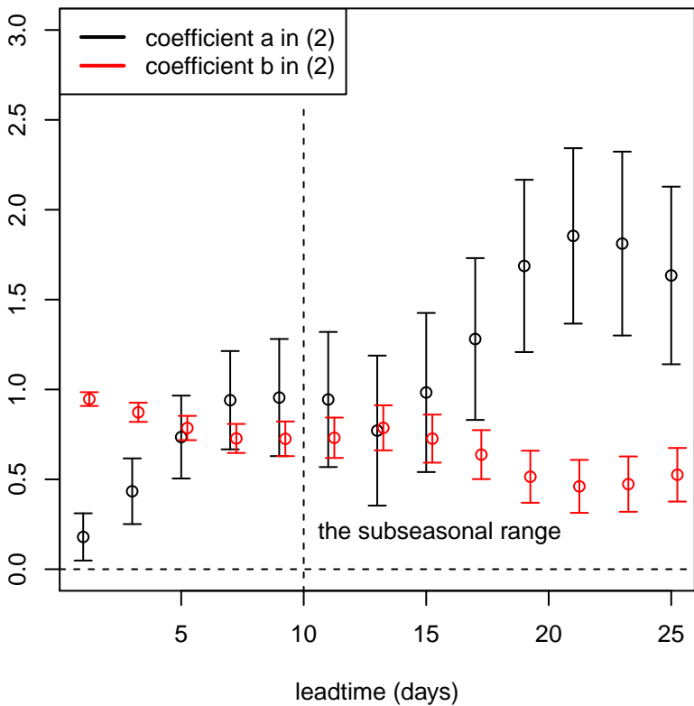
(a) the coefficients of the NGR mean
