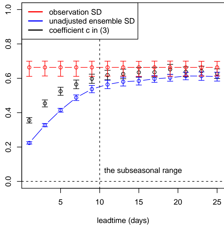
(c) the NGR standard deviation
