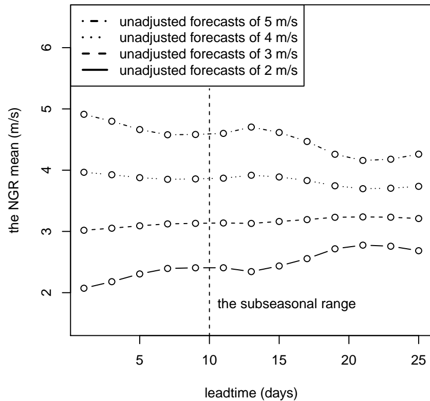
(b) Unadjusted ens. means vs. NGR means
