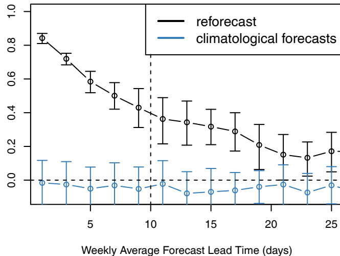
Correlation
