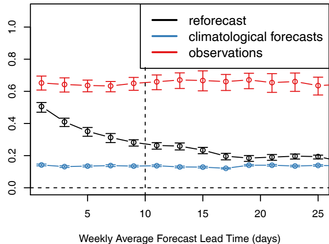
Standard Deviation
