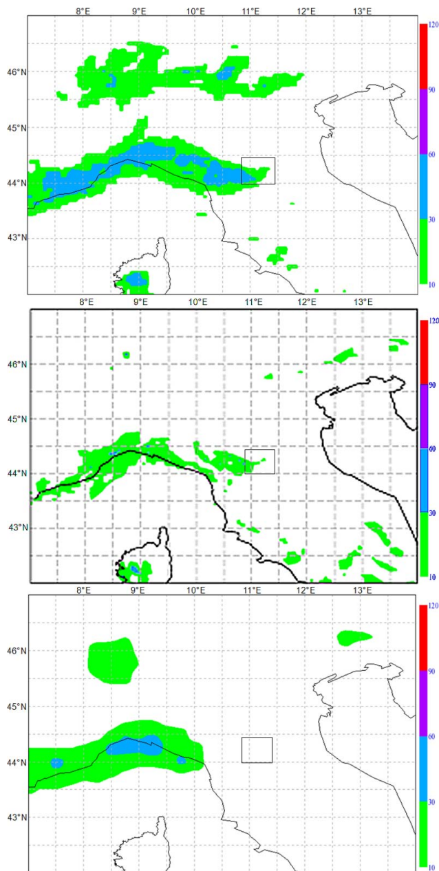
Figure 3. Probability of precipitation exceeding 20 mm/6 h forecast by (from top to bottom) multi-model, COSMO-LEPS and ECMWF EPS, at 00:00 UTC, 30 November 2008. Simulations are initialized at 12:00 UTC, 26 November 2008.
