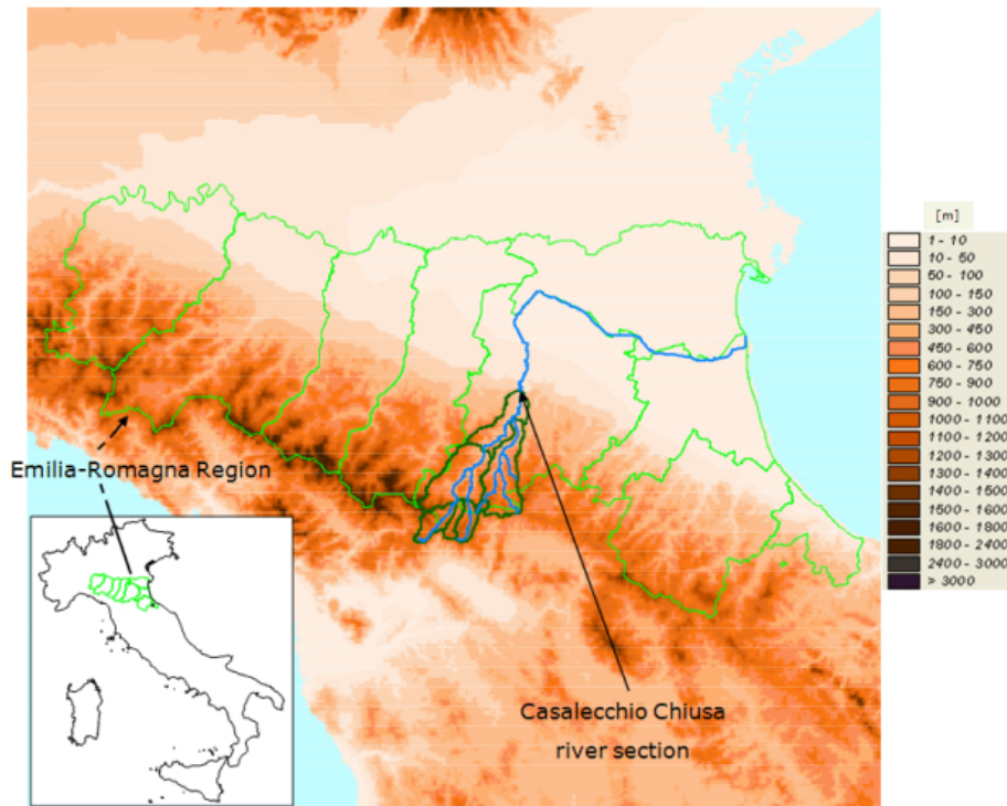
Figure 1. Localisation of the Reno river basin. The main river is showed in cyan. The upper part of the basin, closed at Casalecchio Chiusa, is evidenced with dark green lines.
