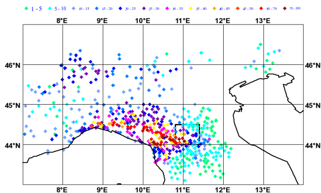
Figure 2. Observed 6-h accumulated precipitation at 00:00 UTC, 30 November 2008. Dark blue diamonds correspond to 20–25 mm/6 h. Black rectangle indicates approximately the Reno river basin.
