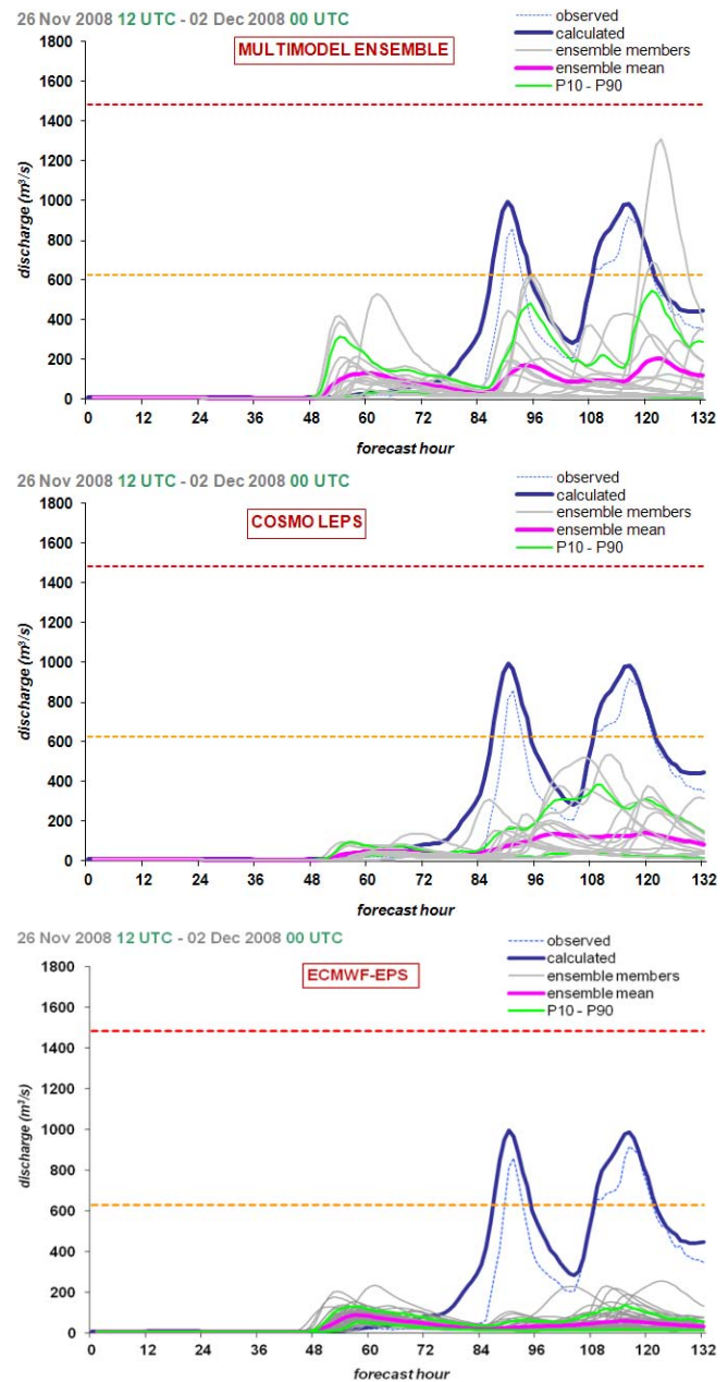
Figure 4. Discharge forecast ( \text{m}^3 \text{s}^{-1} ) vs. forecast range (hours) for multi-model, COSMO-LEPS and ECMWF EPS (51 members), respectively, initialized at 12:00 UTC, 26 November 2008. Each grey line corresponds to an ensemble member. For reference, the observed discharge (dotted blue) and the discharge computed using rainfall observations are provided. Ensemble mean (pink) and the P10-P90 curves (green) are also plotted. Horizontal dashed orange and red lines indicate warning and alarm thresholds, respectively.
